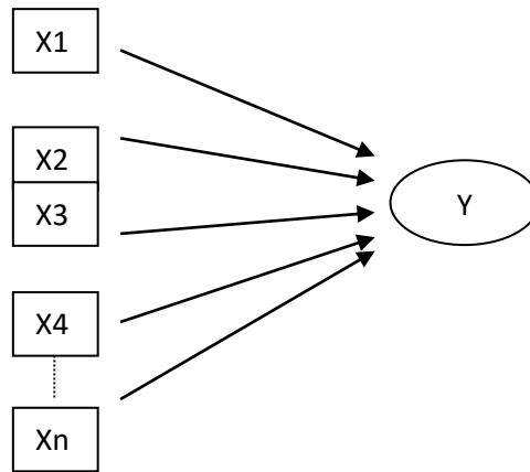
Gambar 2. Model Analisis Regresi
